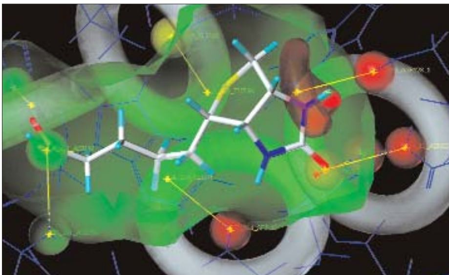
A UNITY query constructed at the active site of the streptavidin/biotin complex (1STP). Yellow lines originate at hydrogen bonding sites of the protein (shown as spheres) and terminate within the spatial constraint for complementary ligand sites. The rotameric positions of hydroxyl and amine H-bond donors are shown as toroidal constraints. A surface constraint at the protein/ligand interface is shown in green. The spatial cap in red accounts for a bifurcated interaction with an Asp carboxyl. Partial match groups are shown in different colors: red, yellow, or green.
